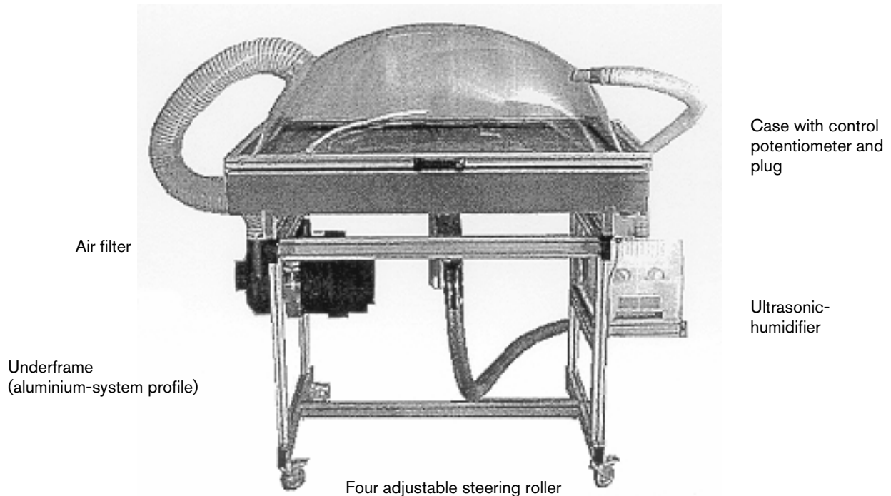
Plexiglas cover
